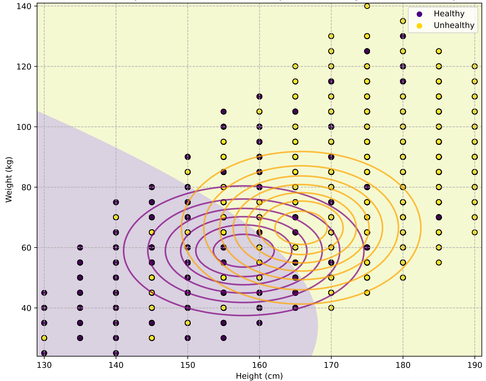
Decision Boundary and Class-conditional Density Contours using Gaussian Naive Bayes
